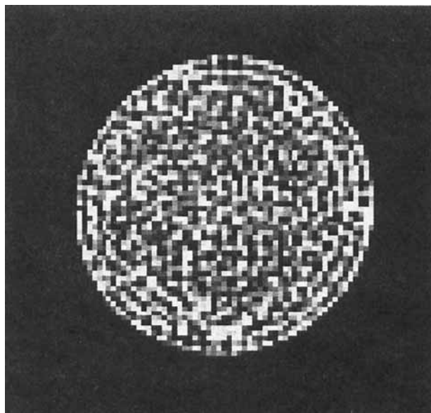
Figure 2. NMR image ( 128 \times 128 pixel) of the ^1\text{H} spin-density distribution in the sphere pack.
