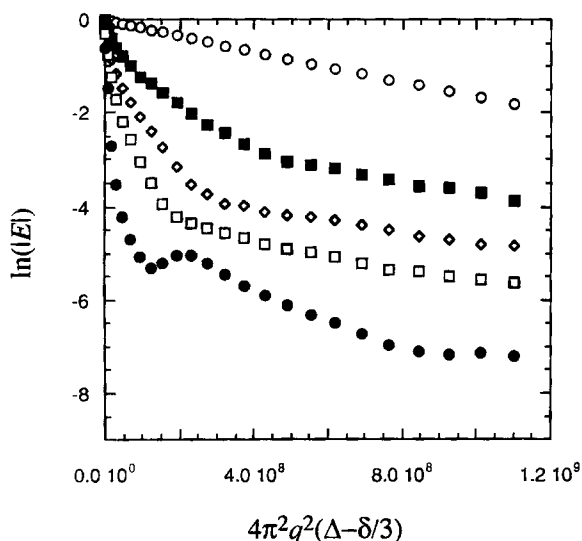
Figure 8. Stejskal-Tanner plot of the natural log of the modulus of the echo-attenuation function, E , as a function of the square of the wave vector.
